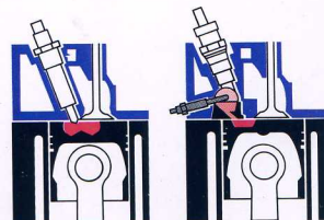
Direct Injection
