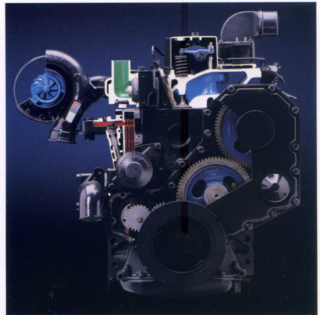
Indirect Injection
